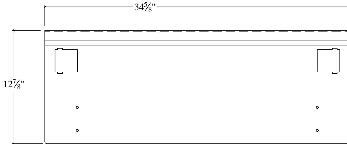
Front View of Comp Cut Tailgate
