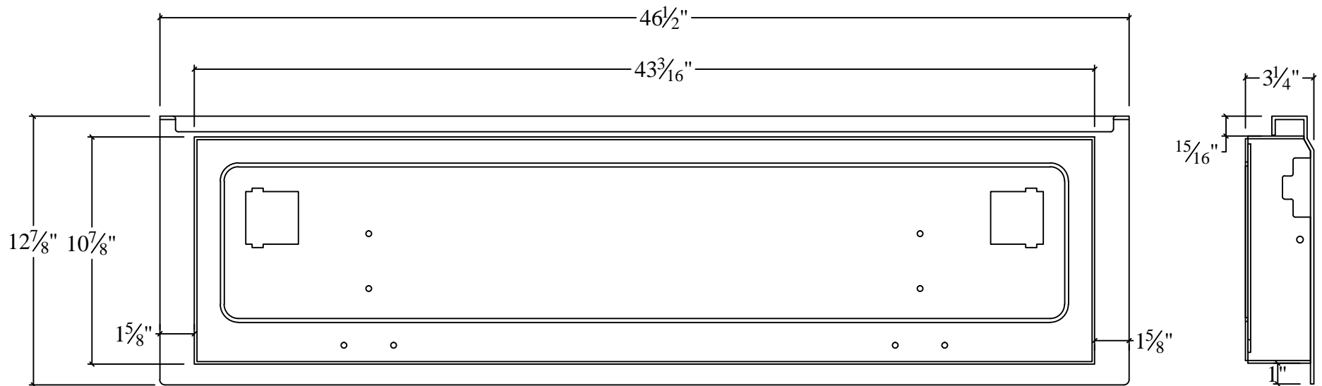
Inside View of Standard Tailgate
